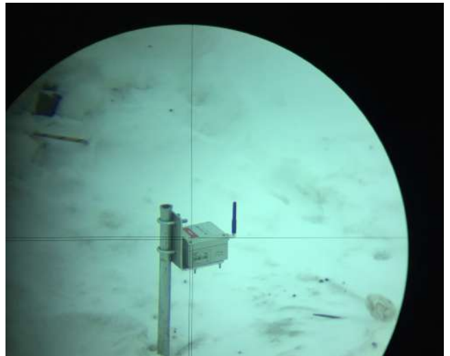
Worldsensing wireless tiltmeter installations
